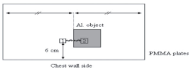
Fig. 2.1 Position of the aluminium filter for the CNR measurement
