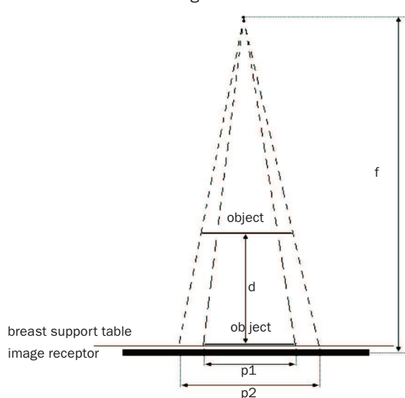
Fig. 2.2 Source-to-image distance measurement
