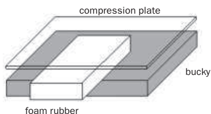
Fig. 2.5 Compression plate alignment measurement, symmetrical load
